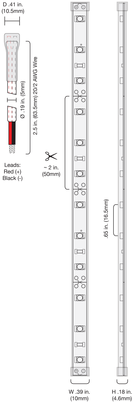
BLAZE™ BASICS 100 Wet Location 12V
