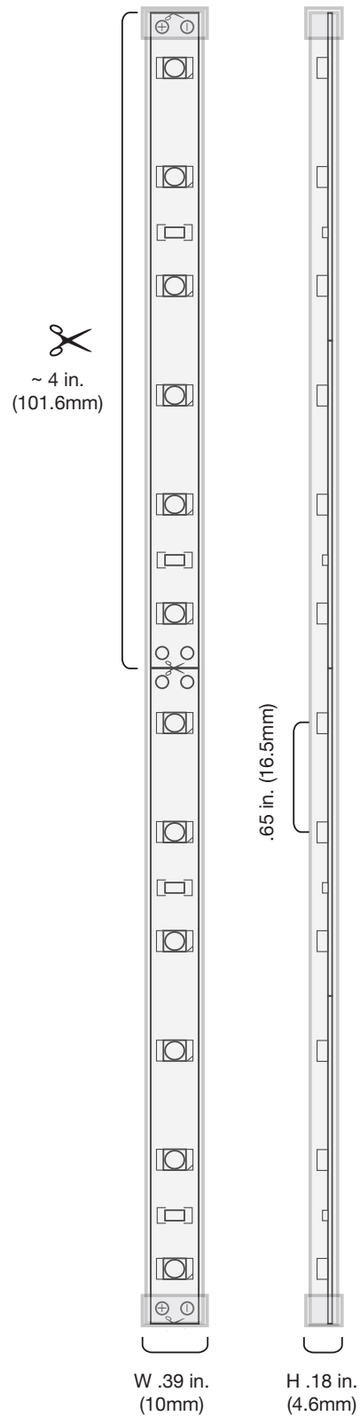
BLAZE™ BASICS 100 Wet Location 24V
